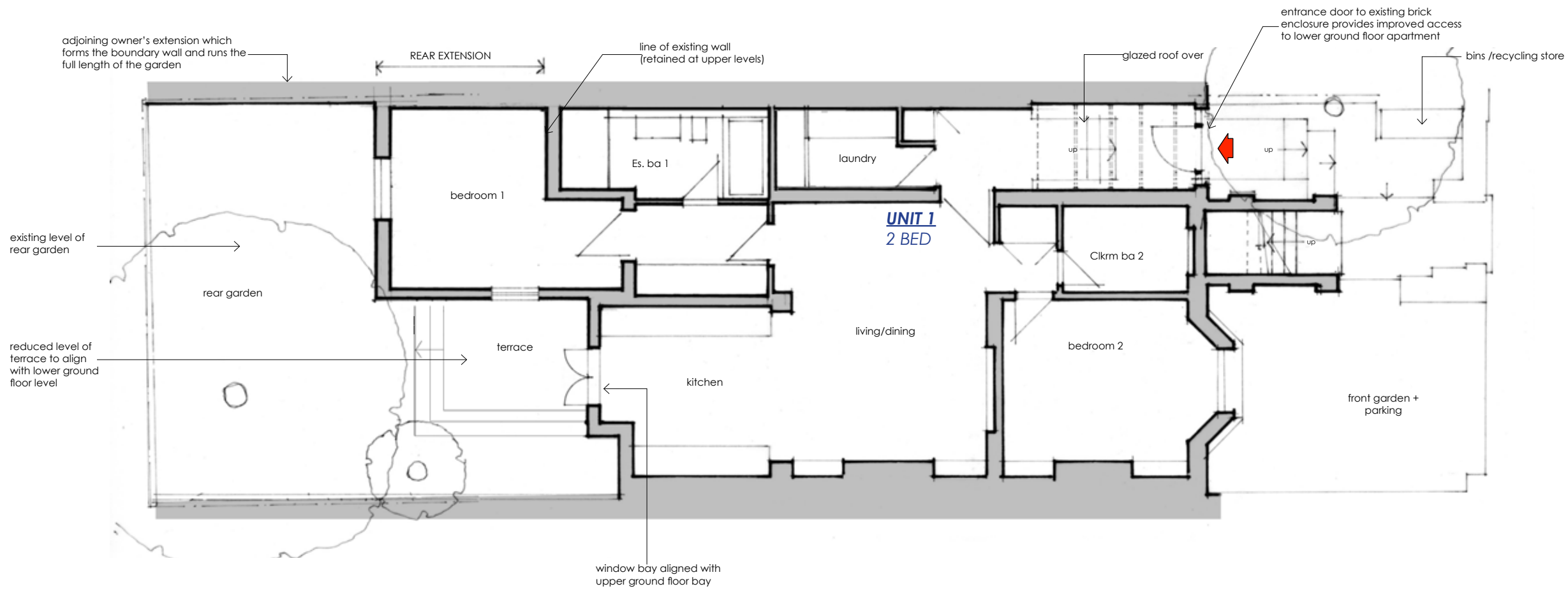
LOWER GROUND FLOOR PLAN - unit 1 (2 bed apartment)
